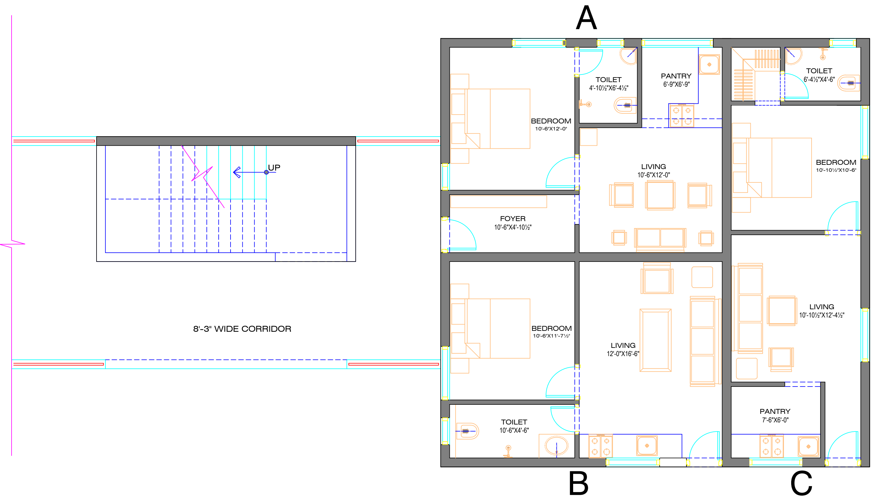
STAFF QUARTER GROUND FLOOR 1524.00 square ft
