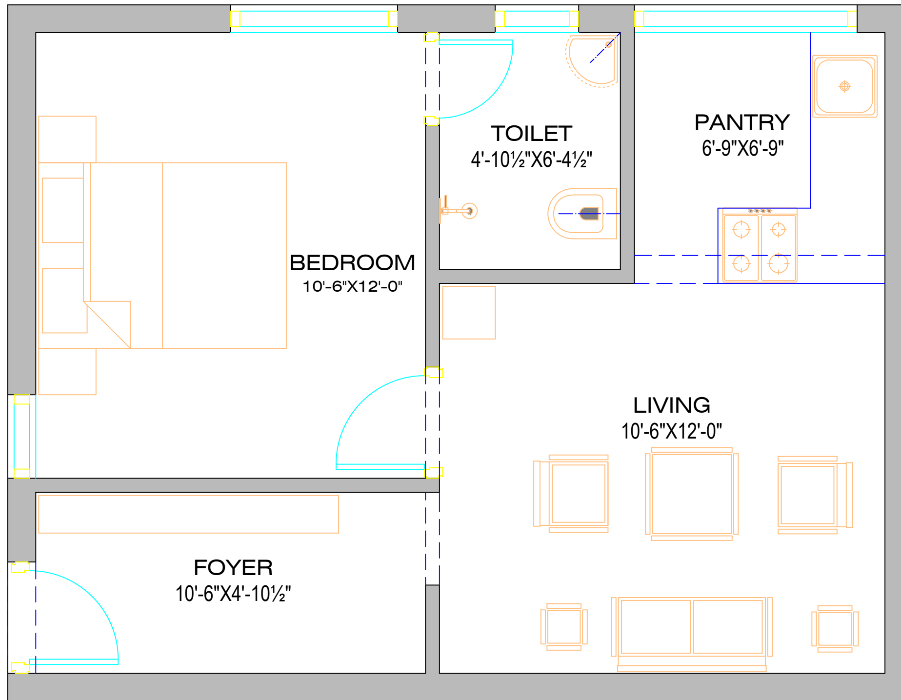
GROUND FLOOR -A 457.00 sft
